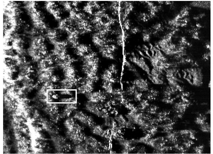
Figure 2. Side-scan sonar image including underwater mine object in bounding rectangle.
